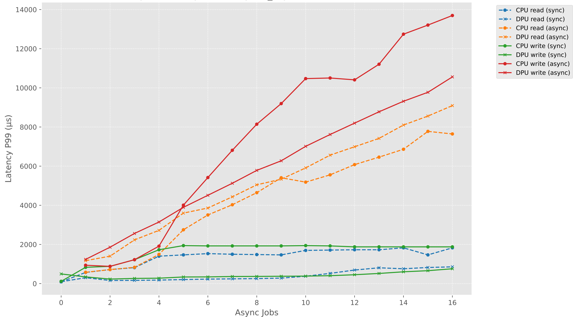
Latency P99 vs Async Jobs (sync1_asyncN) - SEQ (CPU vs DPU)
